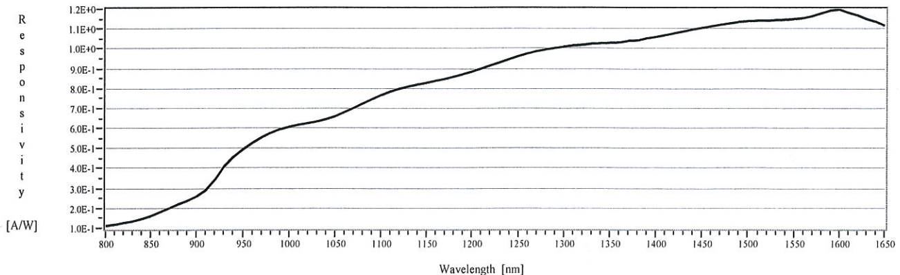
Responsivity versus Wavelength Detector Without External Attenuator
