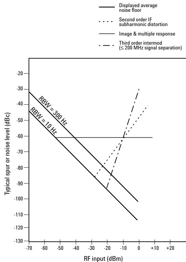
Figure 3. Agilent 11974A System Dynamic Range
