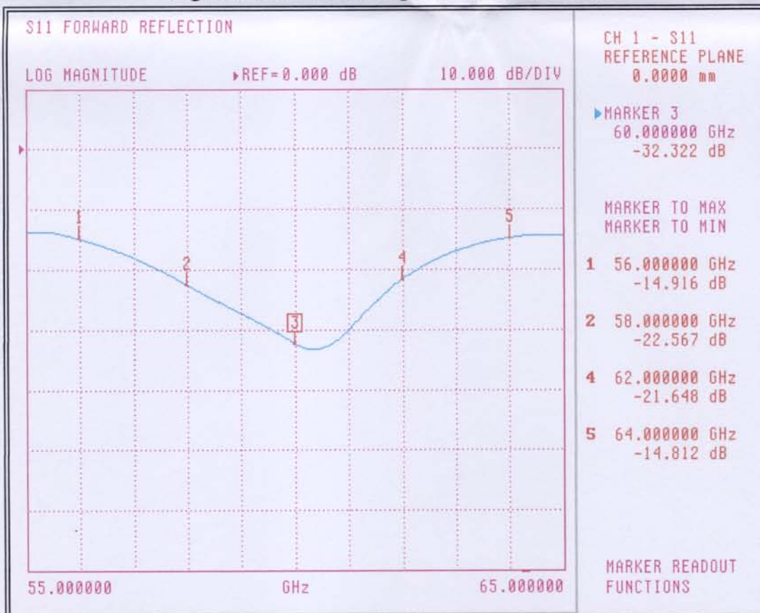
Figure2. Return Loss
