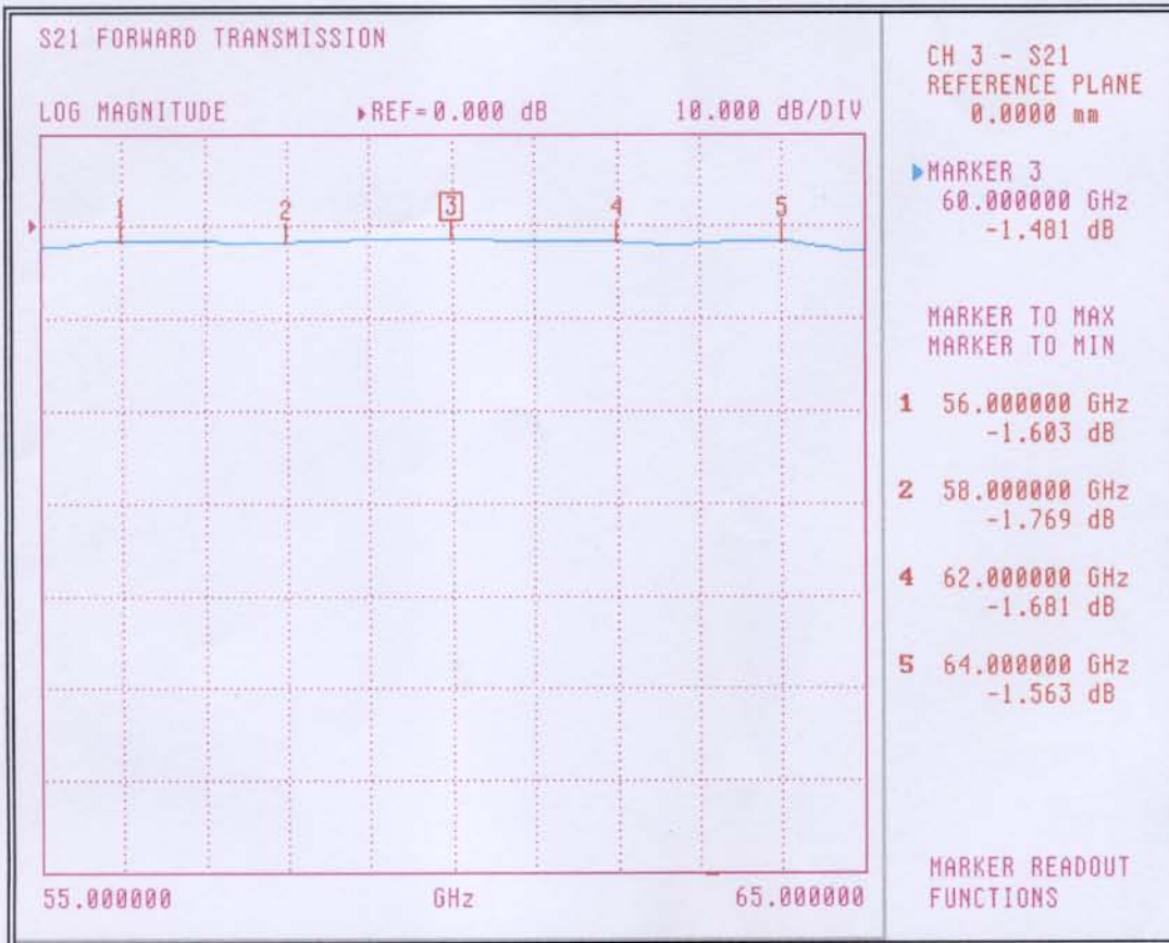
Figure1. WR-15 Waveguide Back to Back
