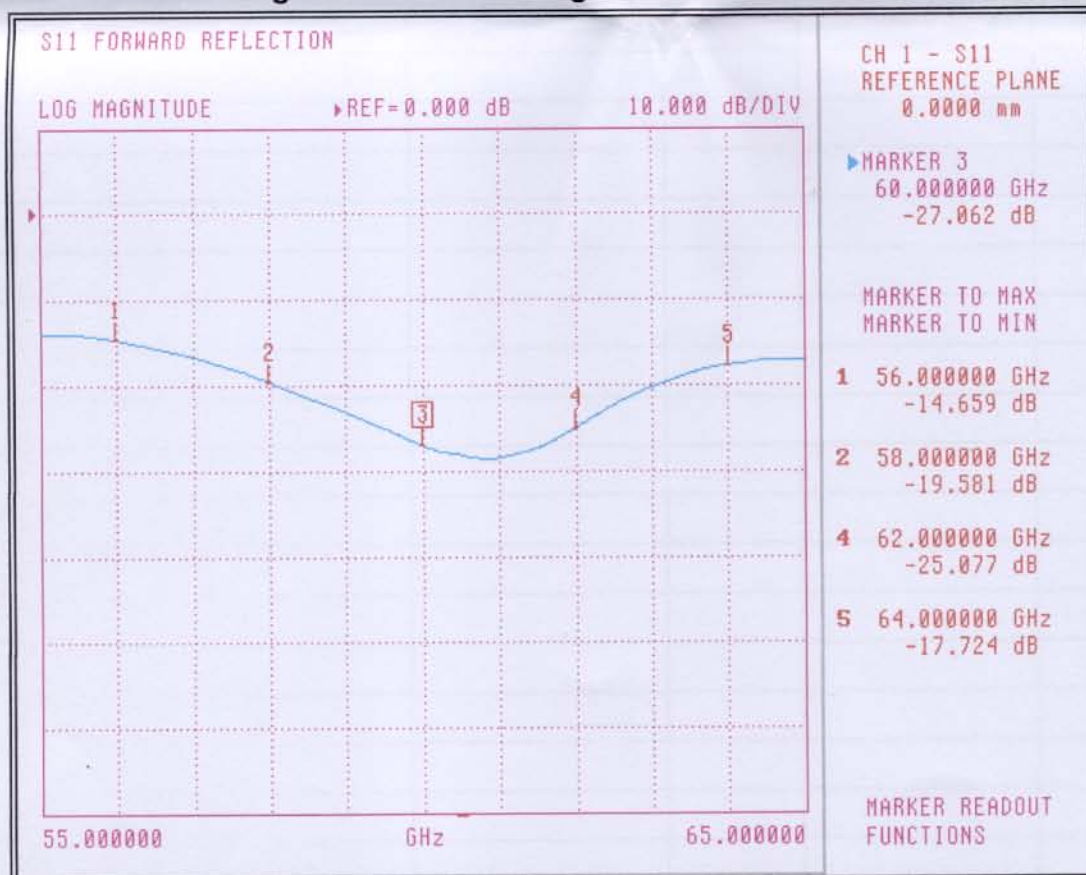
Figure2. Return Loss
