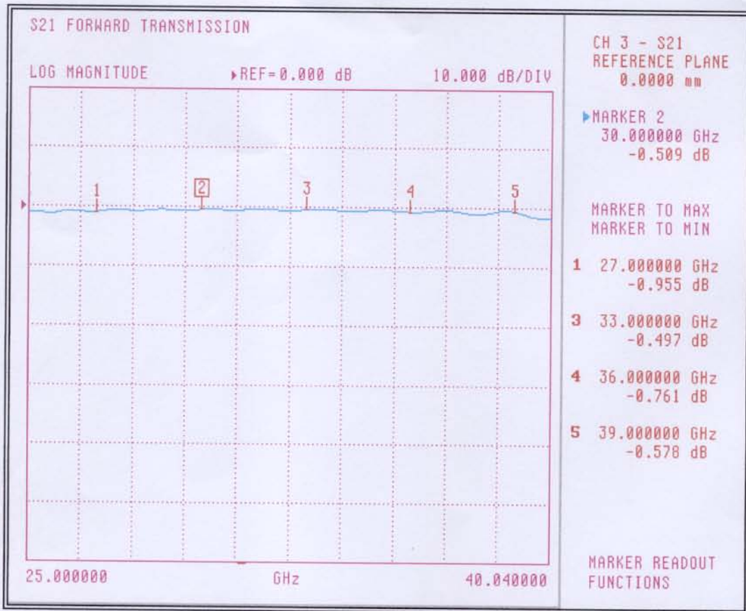
Figure1. WR-28 Waveguide Back to Back
