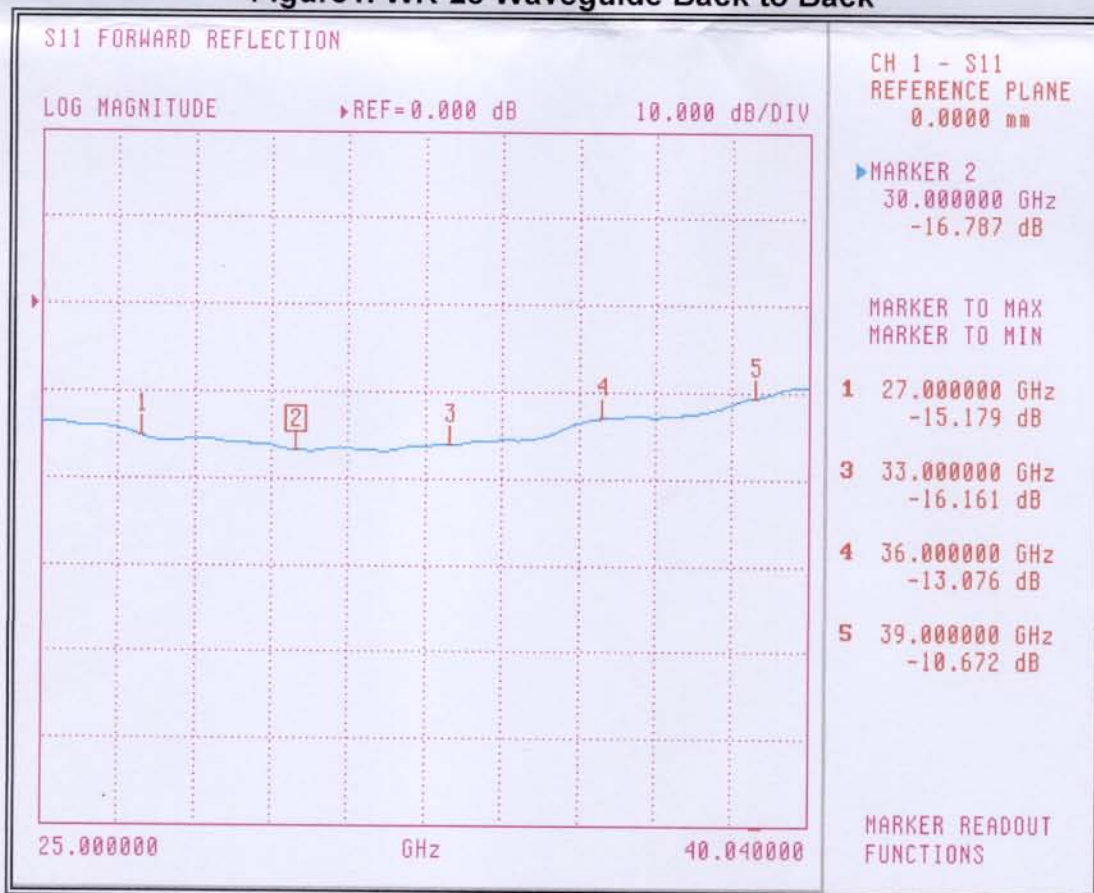
Figure2. Return Loss
