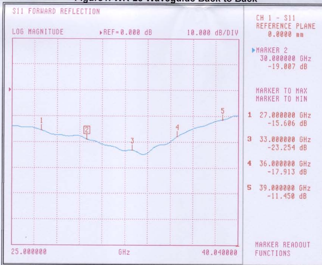
Figure2. Return Loss
