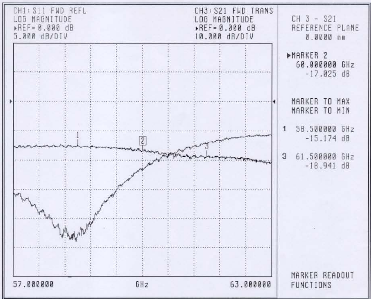
Figure 3-1 S21
