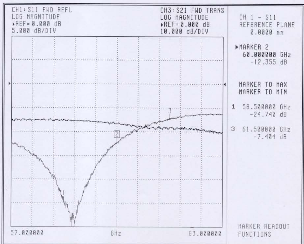
Figure 3-2 S11
