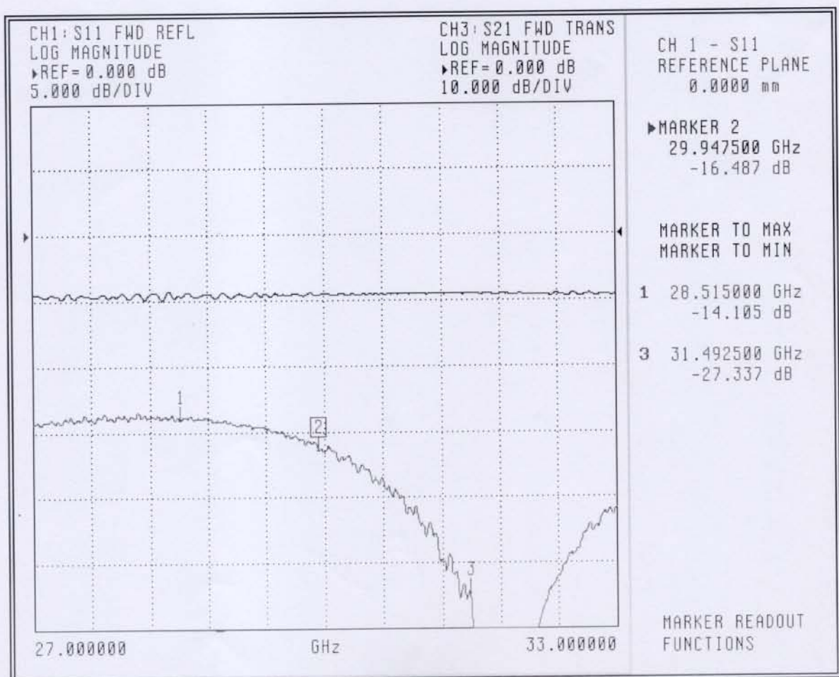
Figure 2-2 S11
