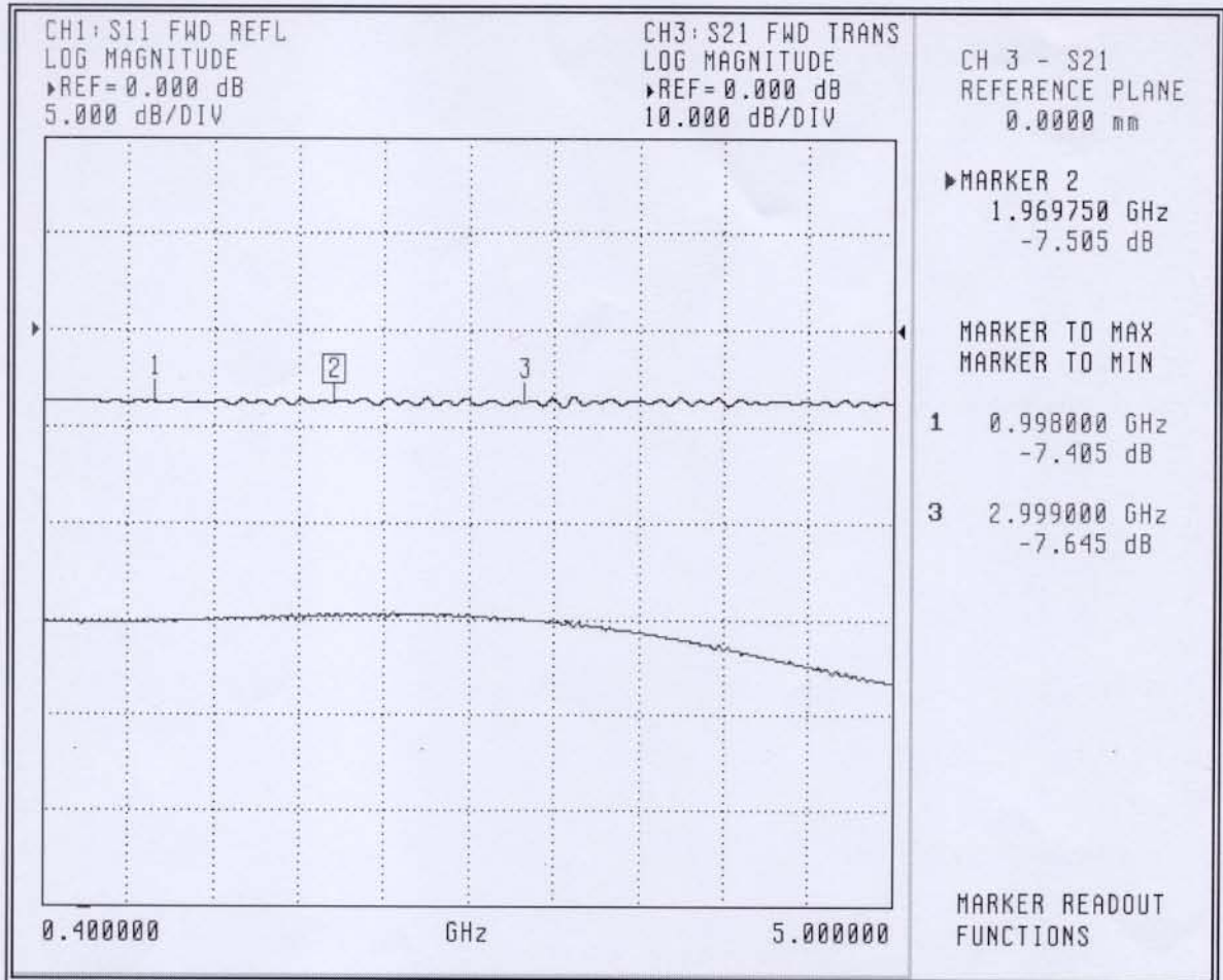
Figure 1-1 S21
