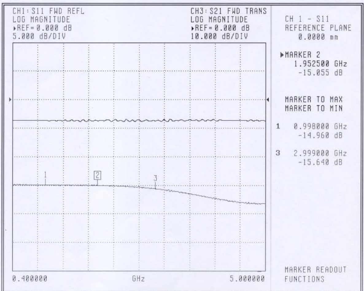
Figure 1-2 S11
