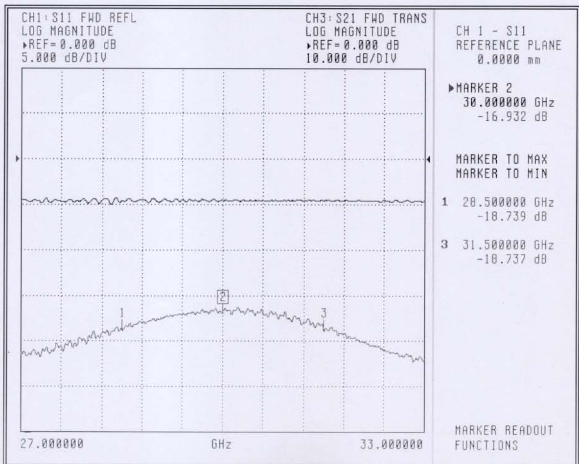
Figure 2-2 S11
