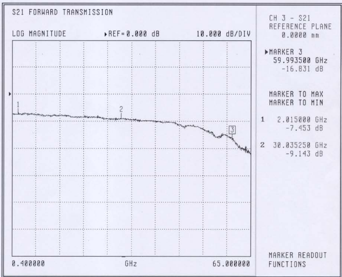
Figure 4 S21
