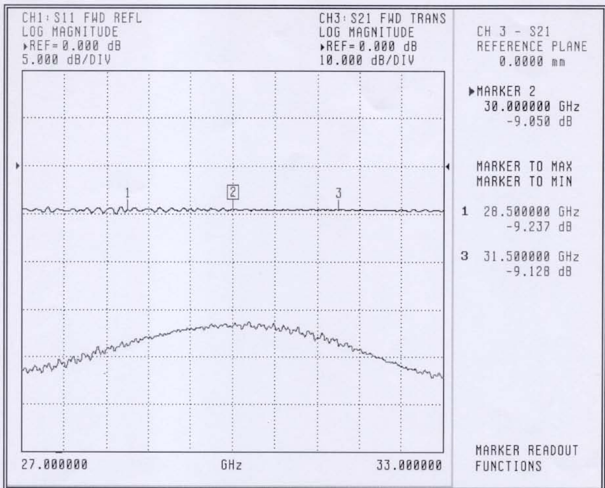
Figure 2-1 S21
