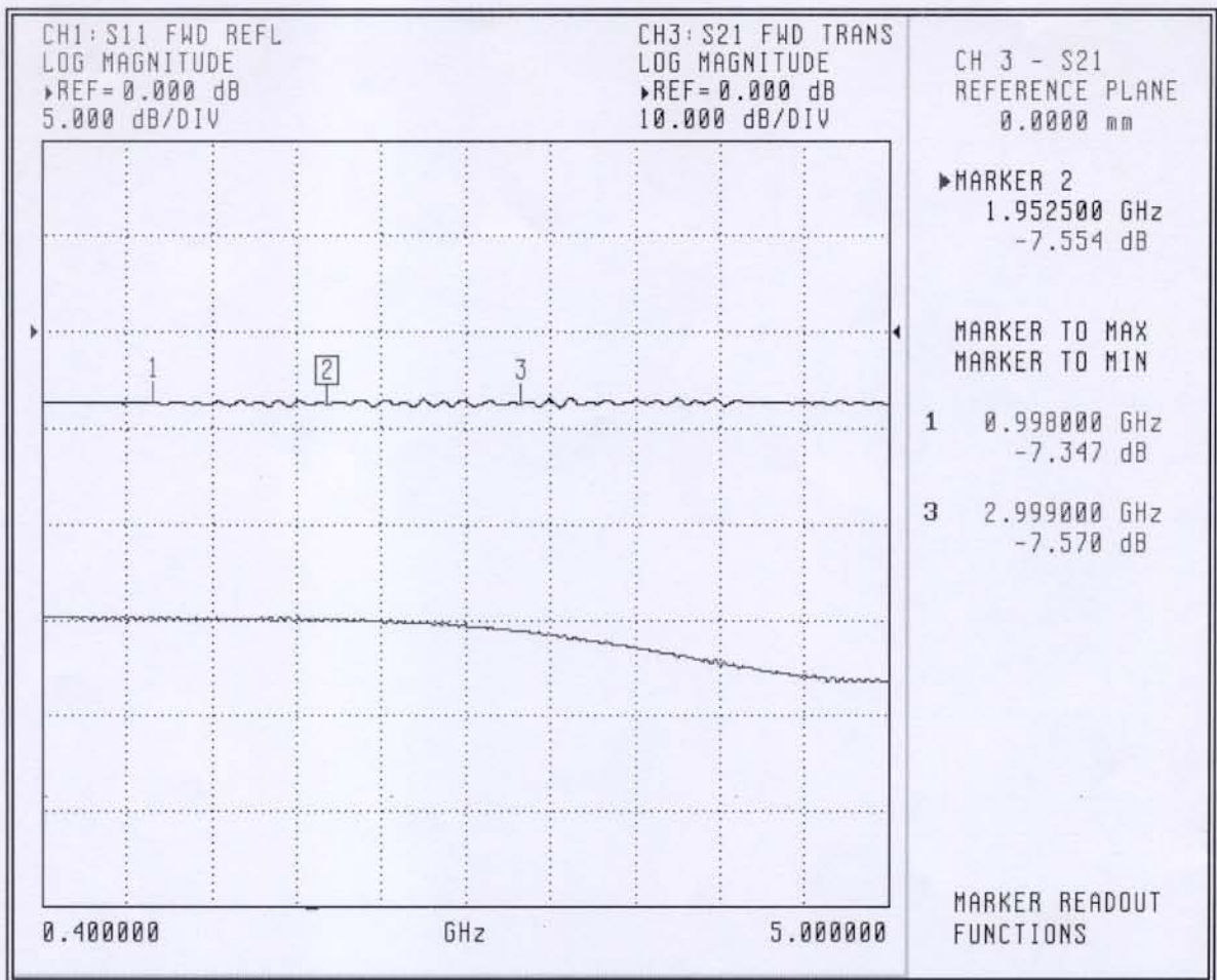
Figure 1-1 S21
