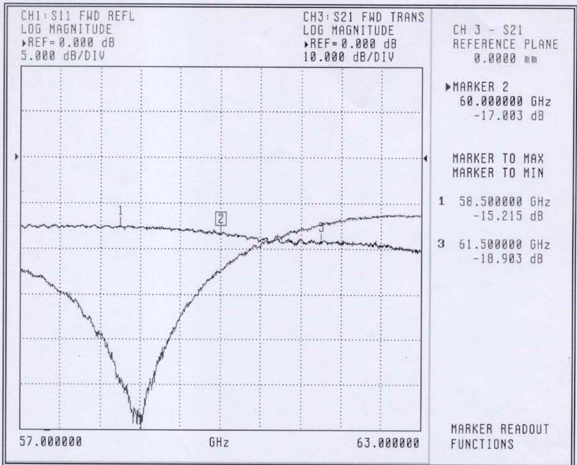
Figure 3-1 S21
