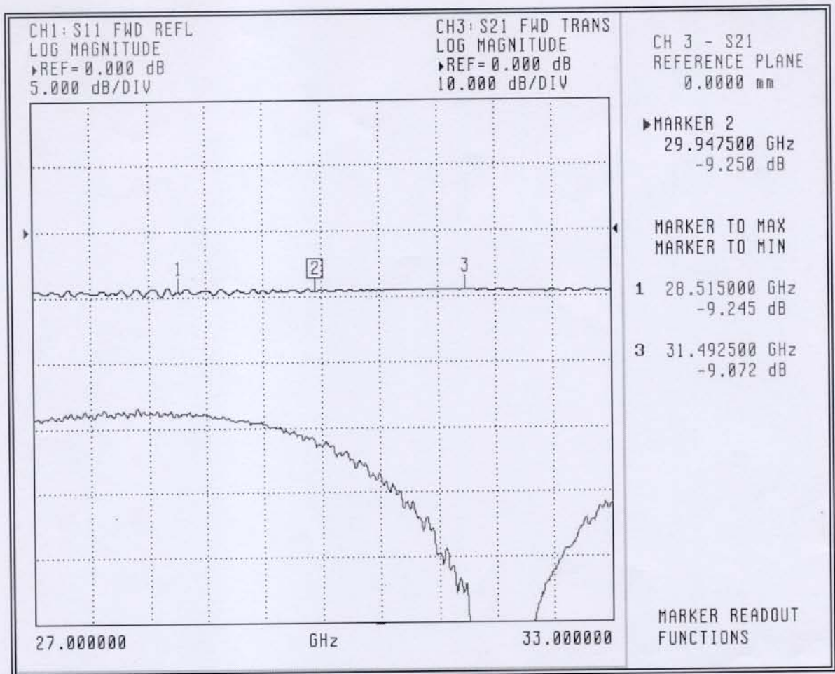
Figure 2-1 S21
