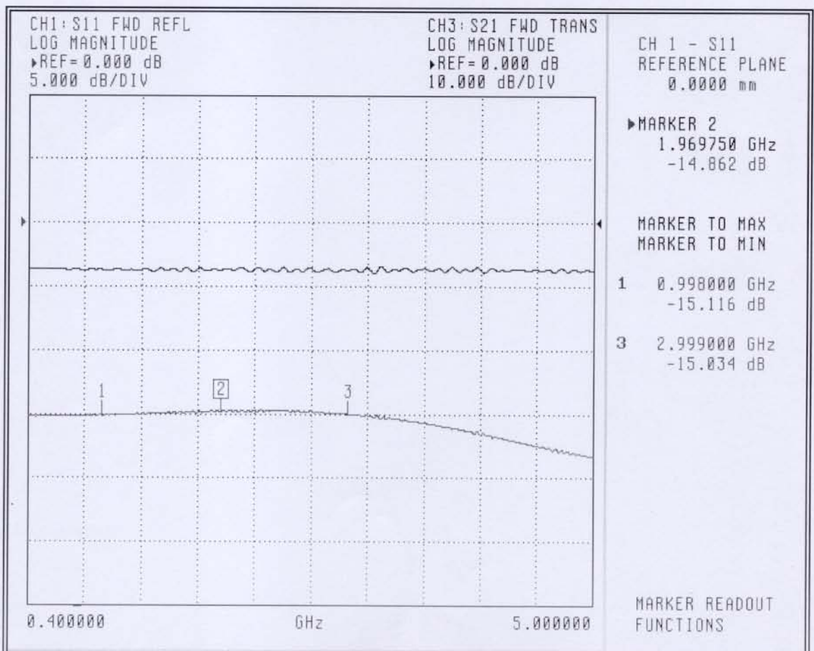
Figure 1-2 S11
