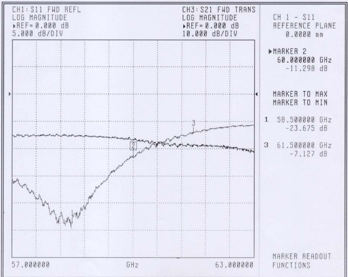
Figure 3-2 S11
