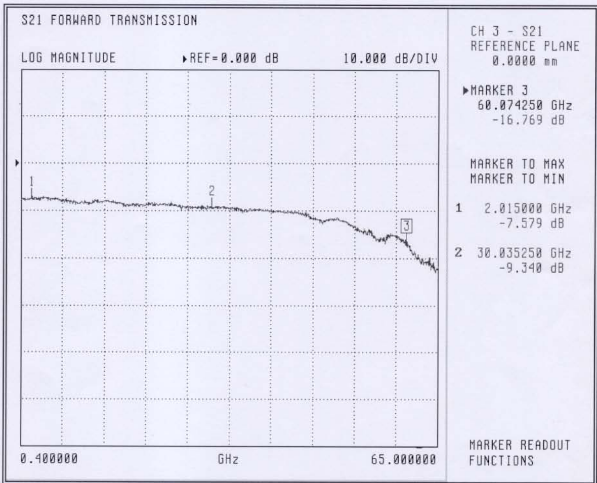
Figure 4 S21
