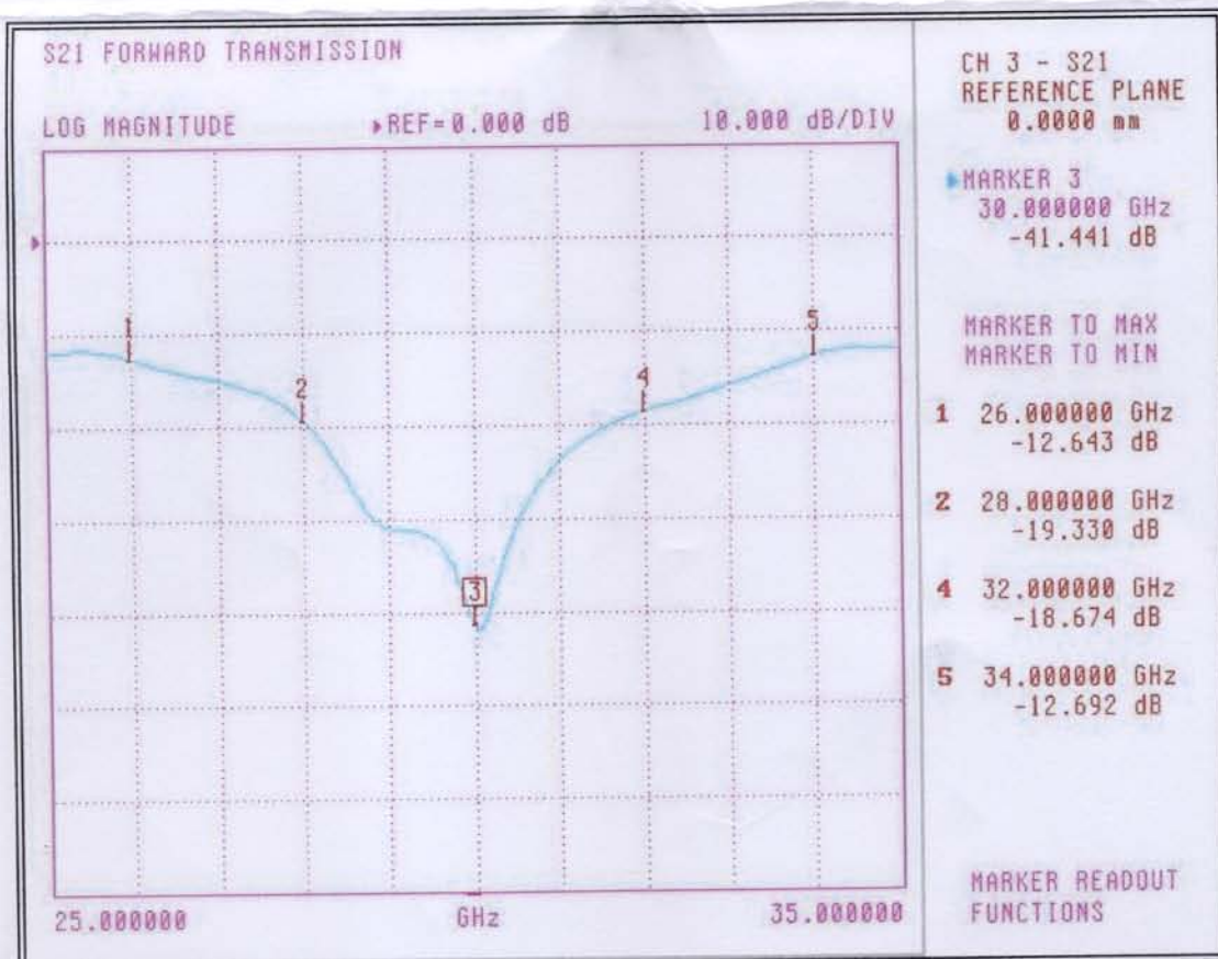
Figure2. Port Isolation
