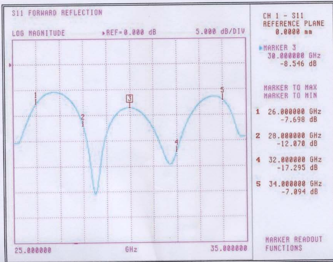
Figure1. Return Loss(S11)
