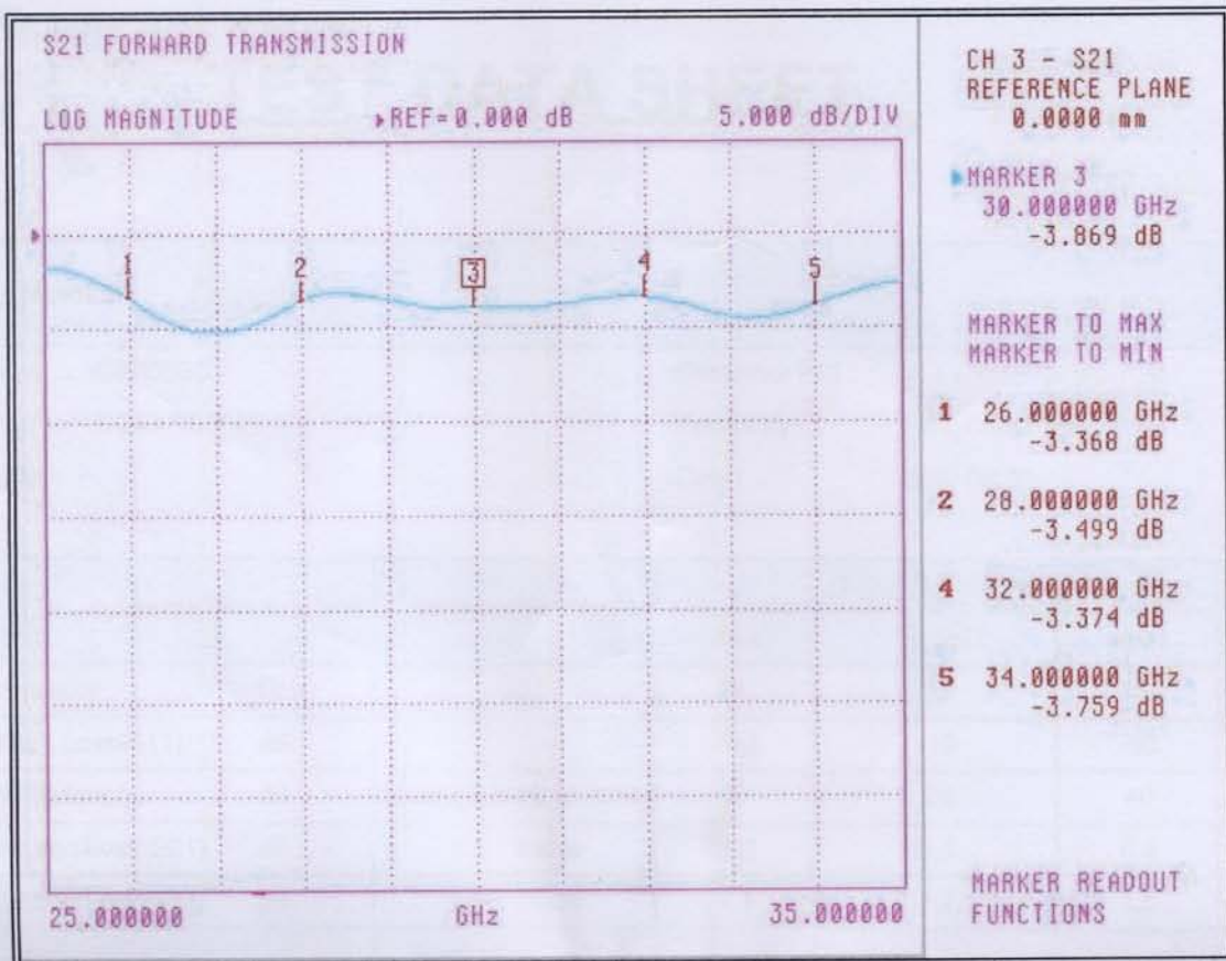
Figure3. Insertion Loss(S21)
