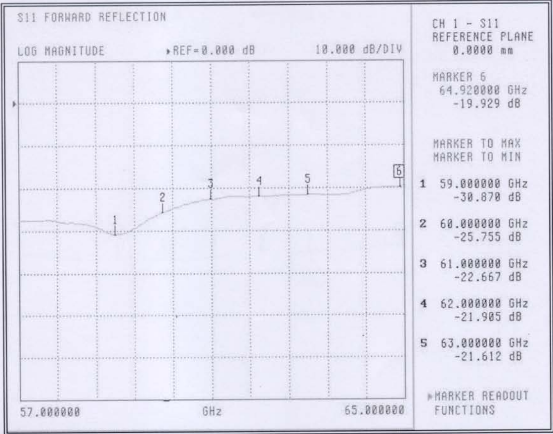
<Fig.1> Return Loss(S11)
