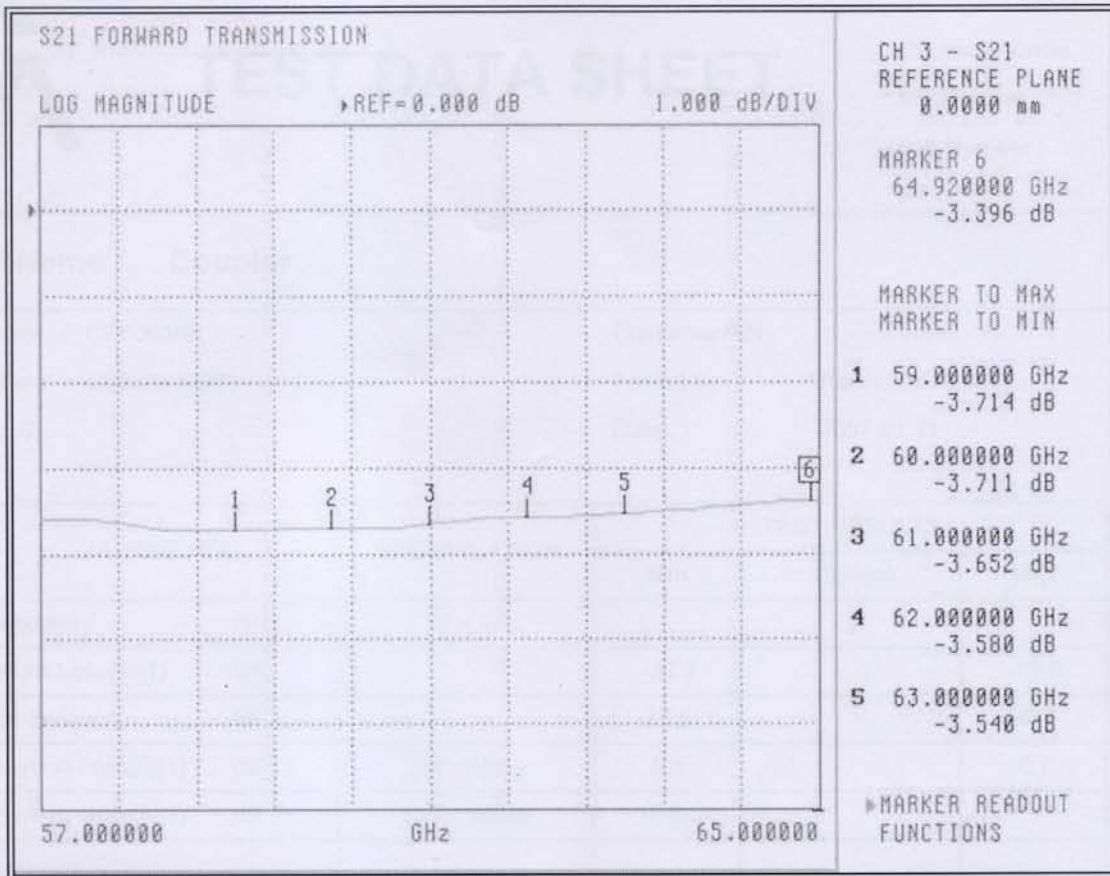
<Fig.3> Insertion Loss(S21)
