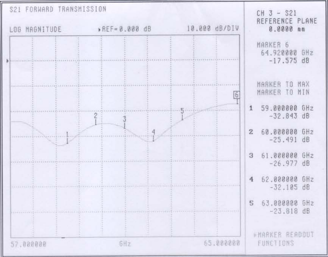
<Fig.2> Port Isolation
