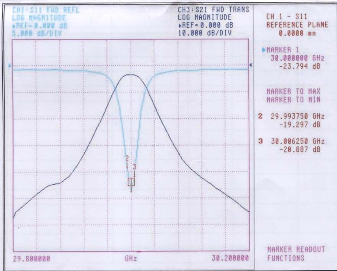
Figure2. S11
