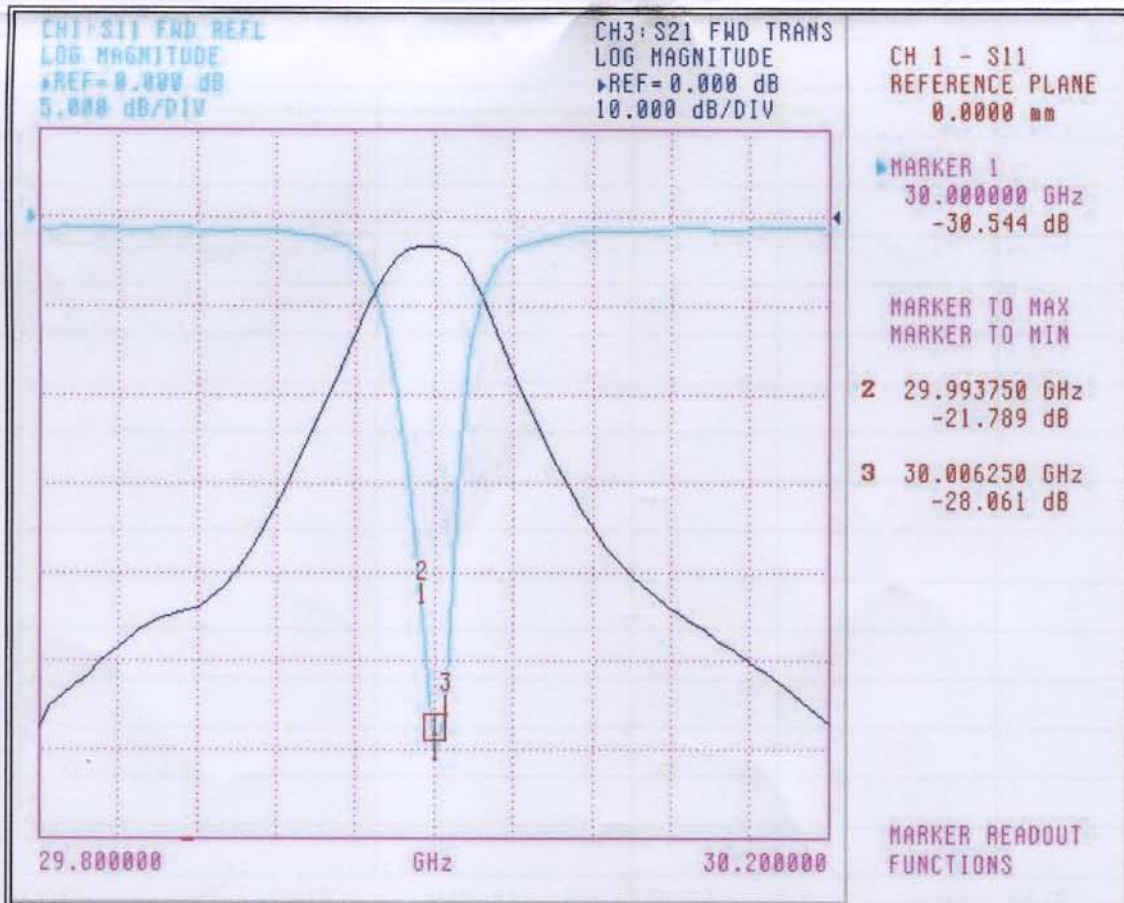
Figure2. S11
