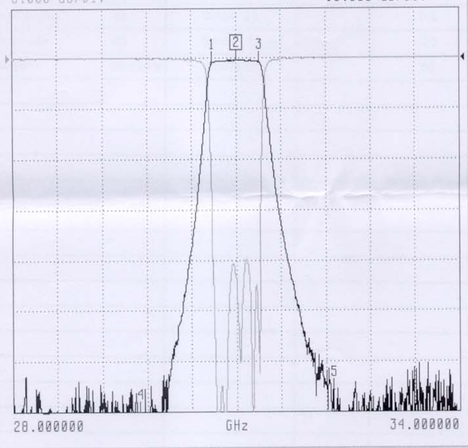
Figure1. S21 & S11
