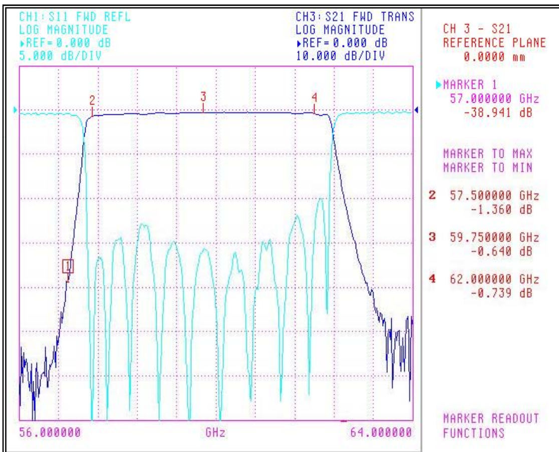
Figure1. S21 & S11
