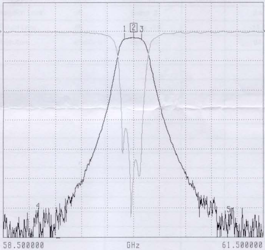
Figure1. S21 & S11
