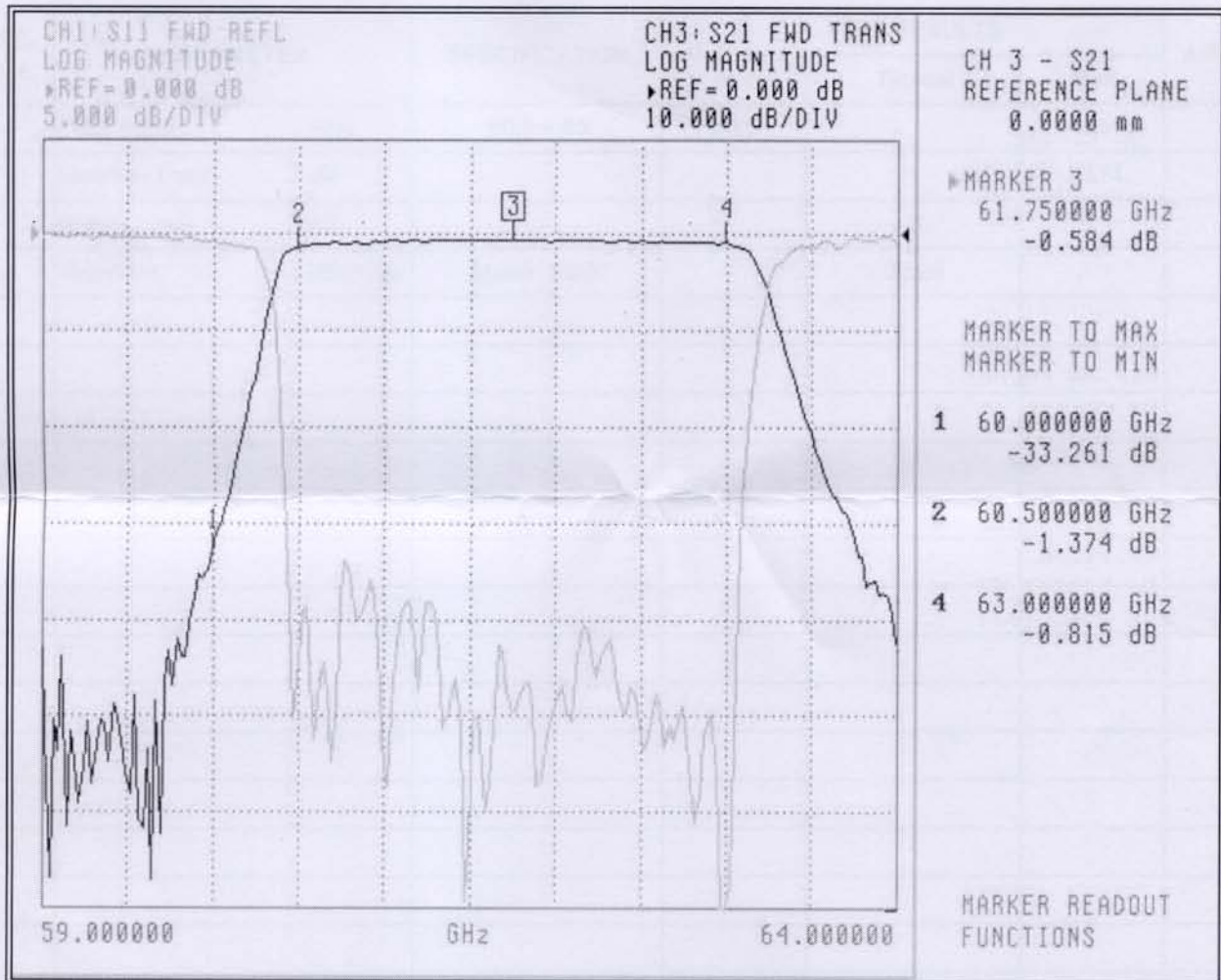
Figure1. S21 & S11
