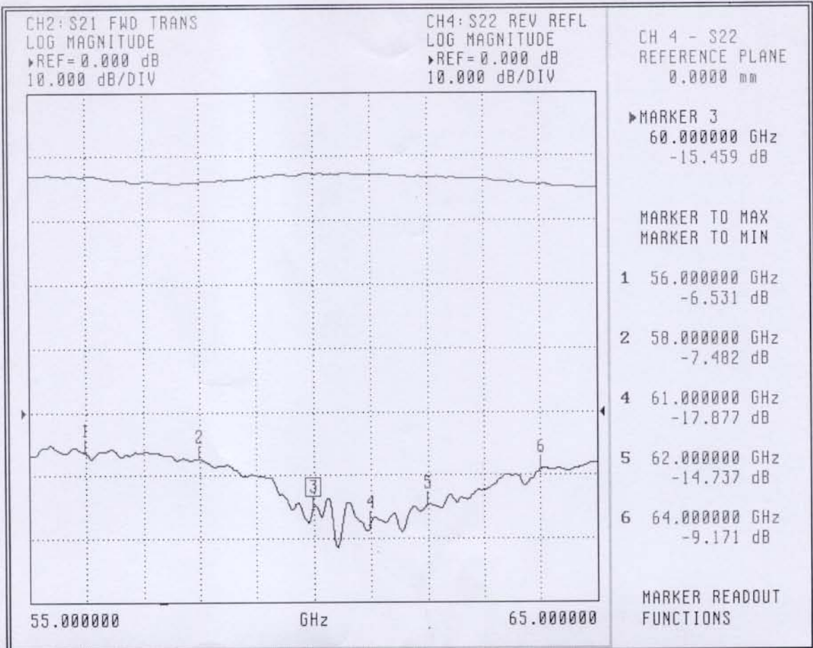
Figure 3. S22
