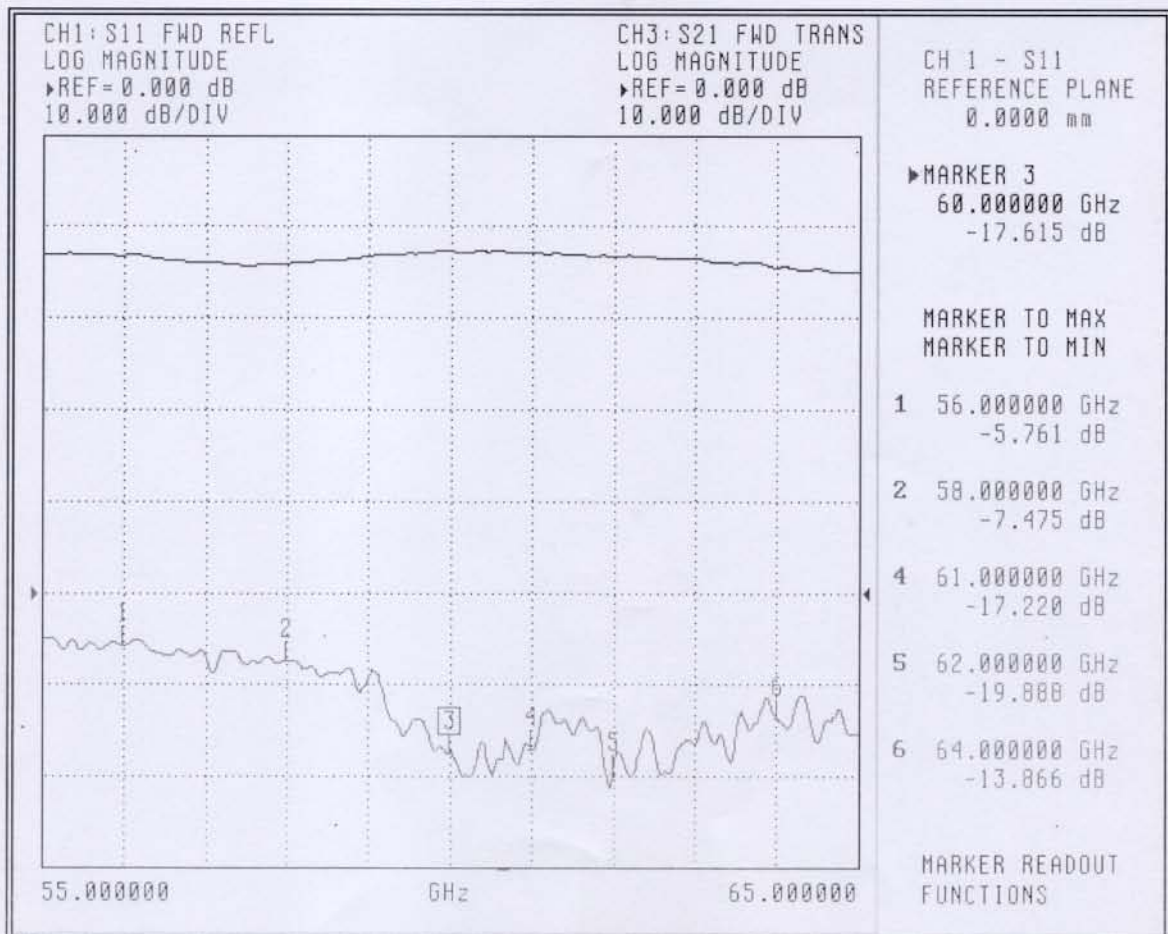
Figure 2. S11
