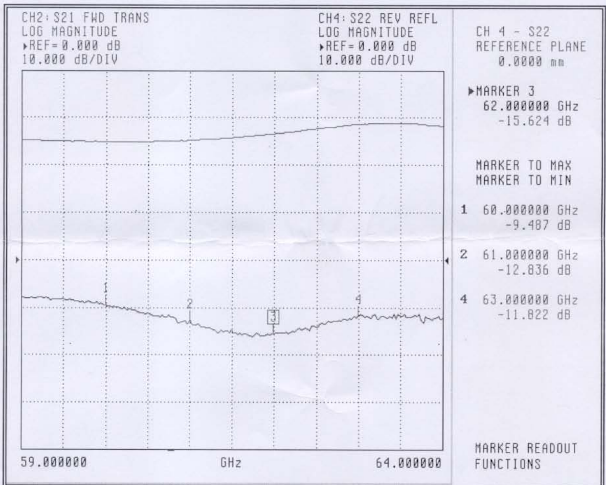
Figure 3. S22
