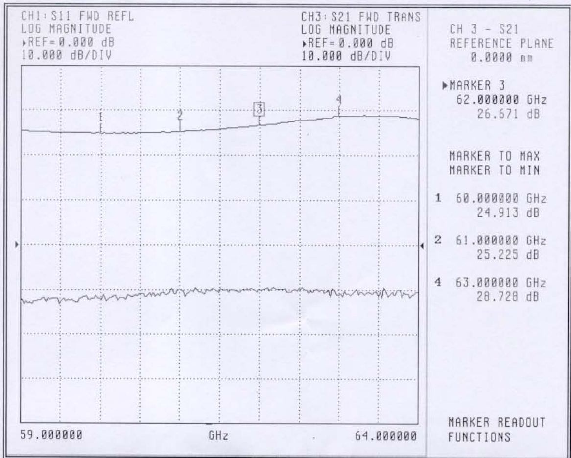
Figure 1. Gain
