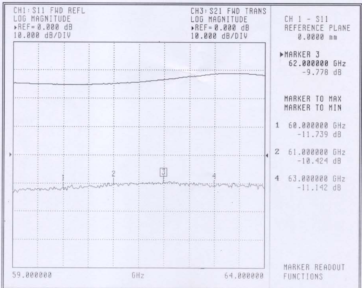
Figure 2. S11
