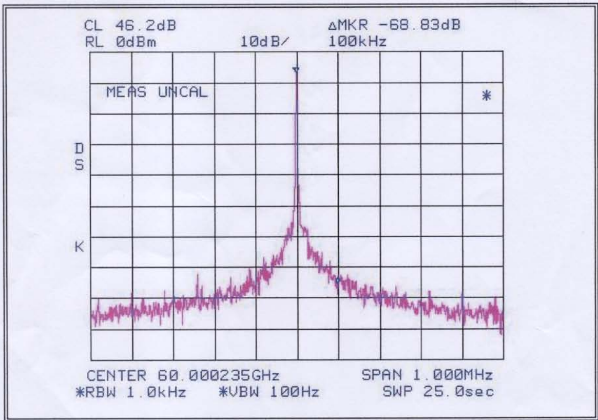
Figure1. PLO Output Frequency
