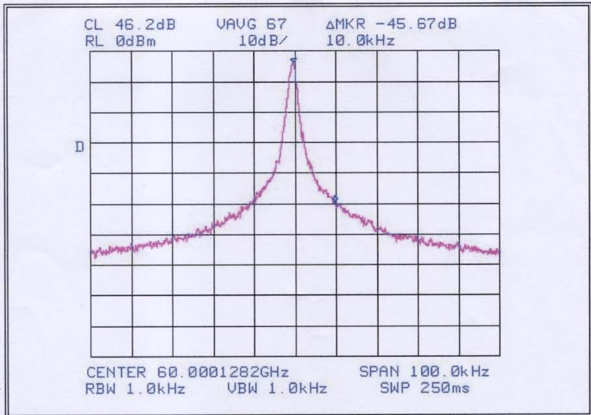
Figure2. PLO Output Frequency
