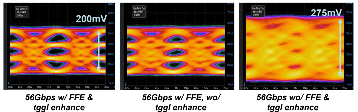
Single ended Driver -4dB channel loss
