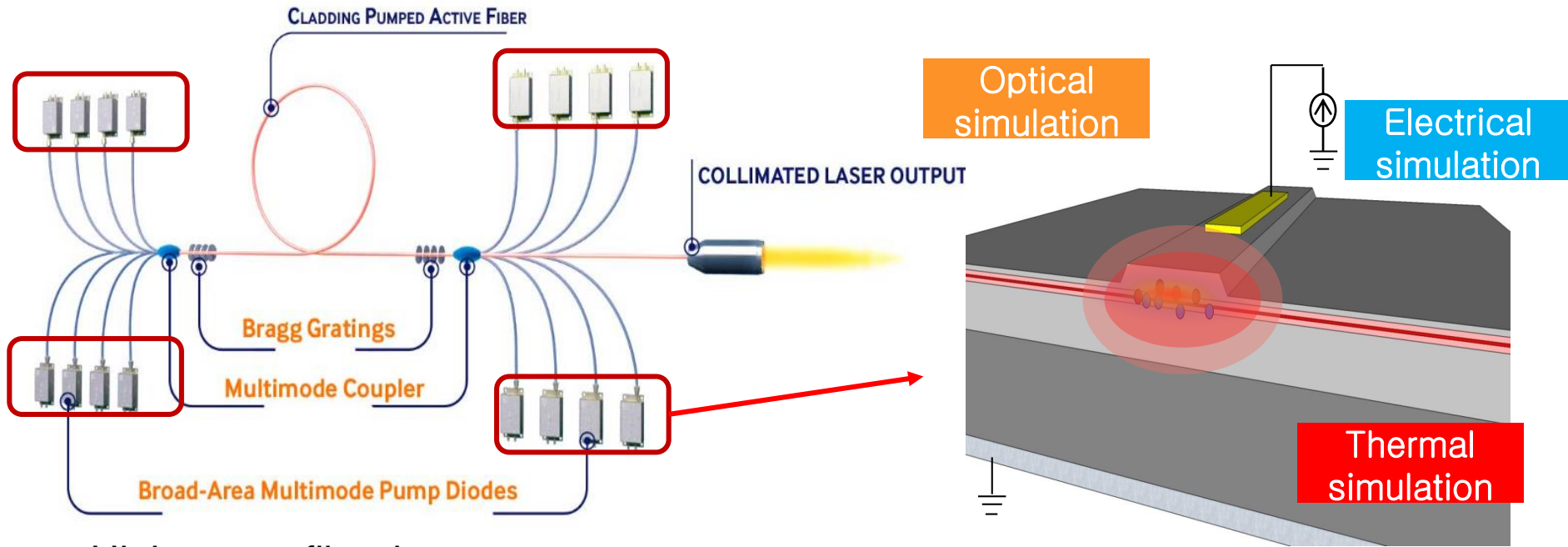
High power fiber laser system
